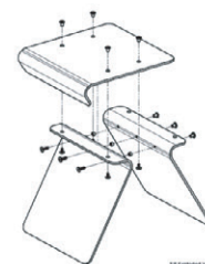
1.0 Exploded View
