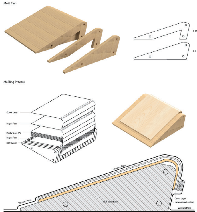
Details of MDF Mold and Vacuum Form Setup
